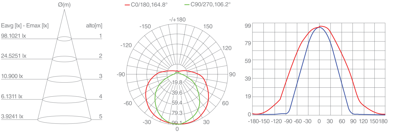
Listón T5 LED
