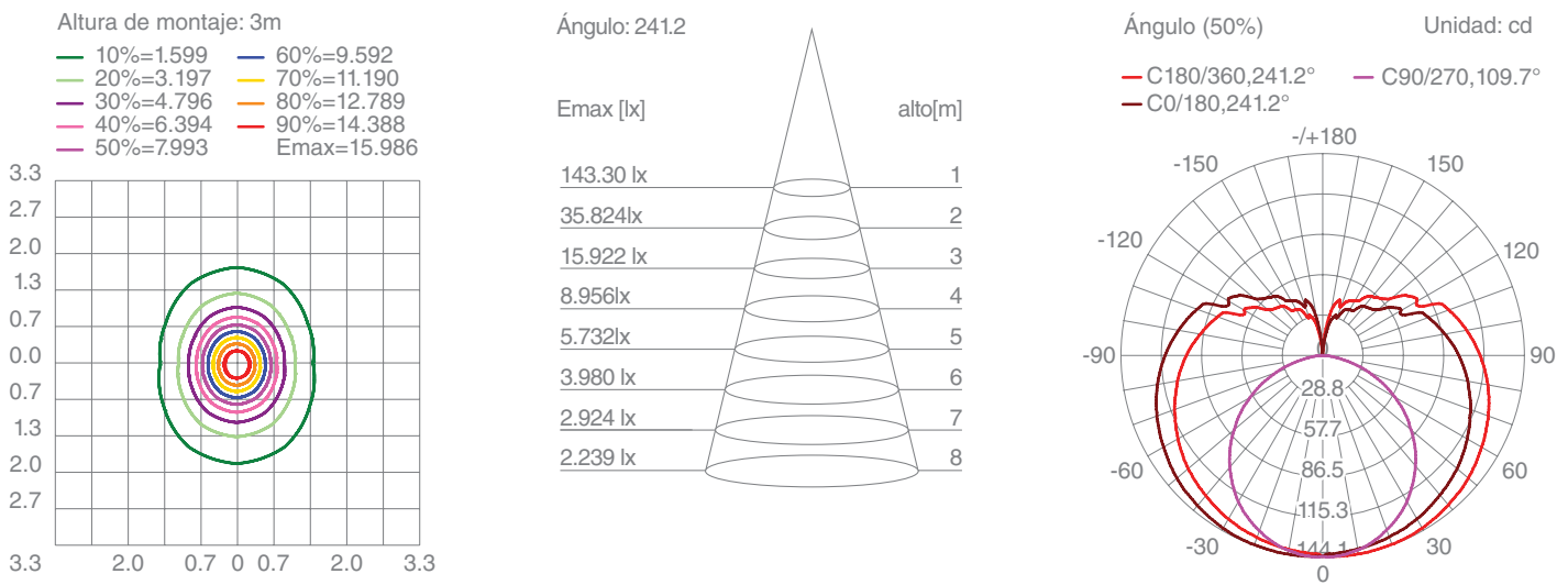
Tubo Led 18W
